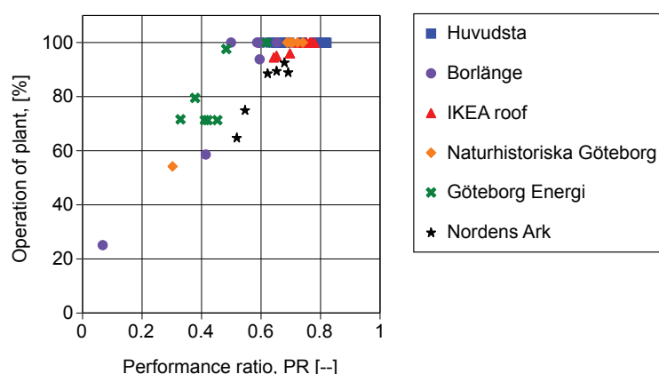
Figure 50, Comparison of the performance to the operation of the plant, six PV plants in Sweden.
