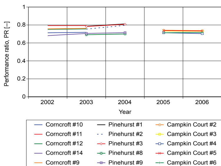
Figure 58, Performance over Time.
