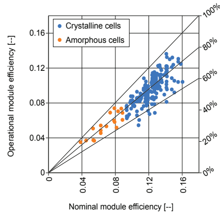
Figure 26, Nominal efficiency to the operational efficiency.
