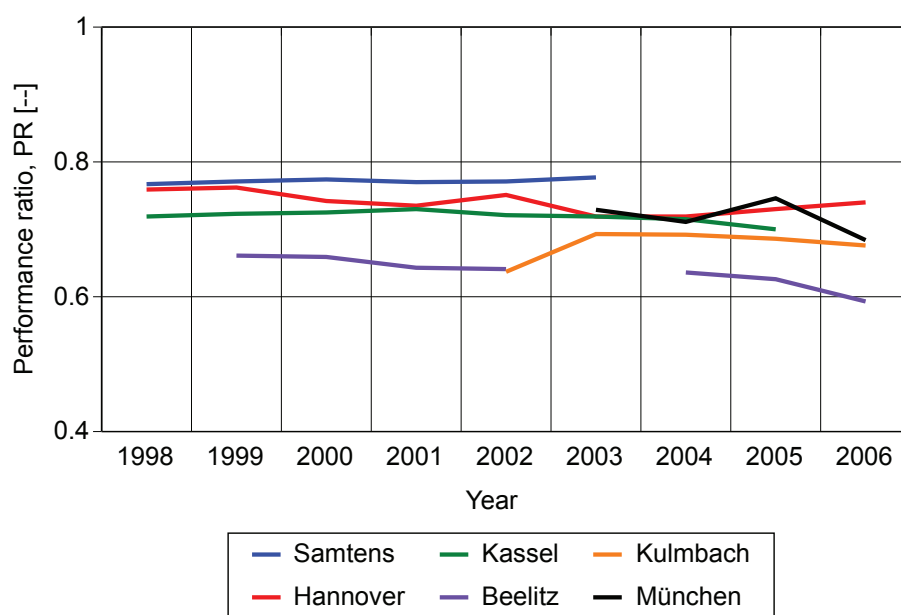
Figure 42, Annual performance ratio over time for six German PV systems (1998 – 2006).
