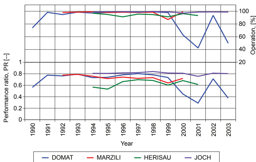
Figure 54, Operation and performance over time, four Swiss PV plants.
