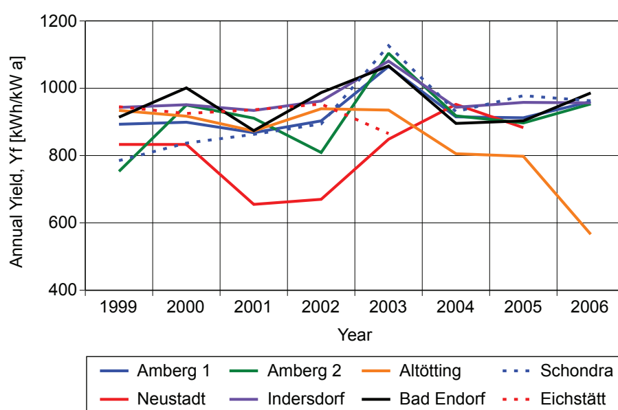
Figure 41, Annual yields of eight German grid-connected PV school plants over eight years of operation (1999 – 2006).
