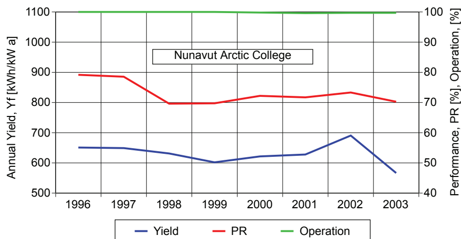
Figure 36, Annual yield, Performance and Operation of the Nunavut Arctic College PV system from 1996 to 2003.
