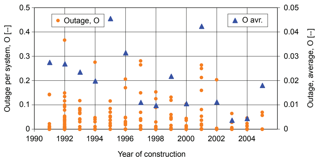
Figure 35, Reported outage ( O ) over time for all the systems and as an average value per year.
