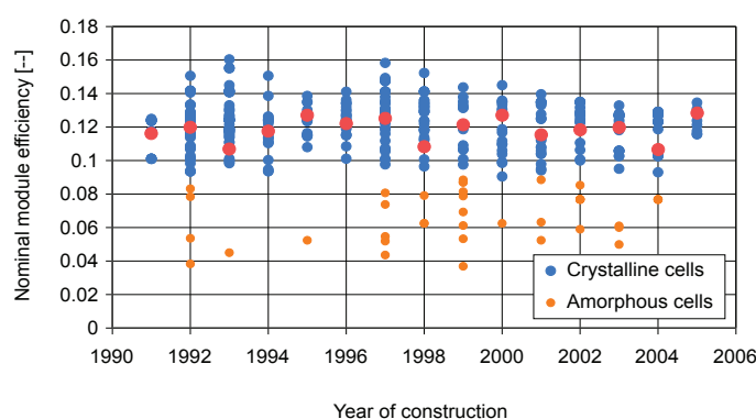
Figure 24, Nominal module efficiency over time.
