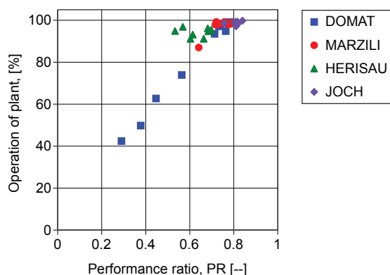
Figure 55, Comparison of the performance to the operation of the plant, four Swiss PV plants.
