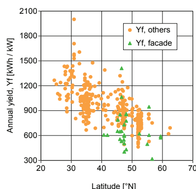
Figure 23, Annual final yield (Yf) vs. northern latitude.
