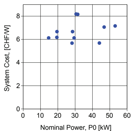
Figure 52, Specific cost in relation to the size of the plant of the 11 PV systems in Figure 51.
