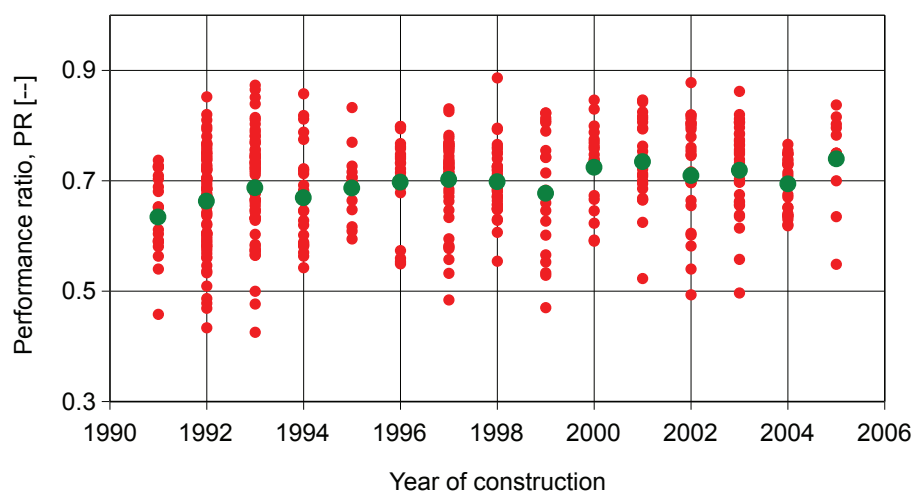
Figure 32, Performance ratio (PR) over time, all data.
