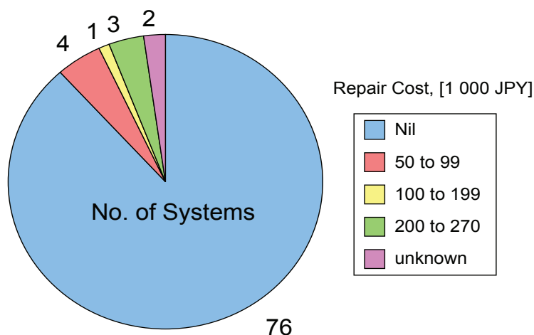
Figure 43, Distribution of the actual repair costs (in 1 000 JPY) from 86 reported cases of 725 Japanese PV systems.
