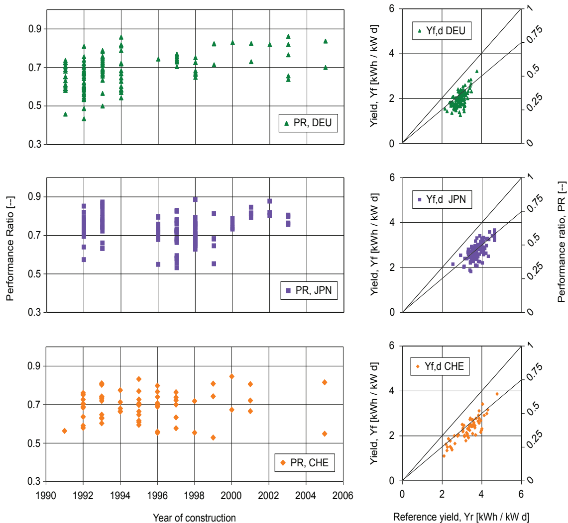
Figure 33, Performance ratio (PR) over time and final yield (Yf) vs. reference yield (Yr) for Germany, Japan and Switzerland.
