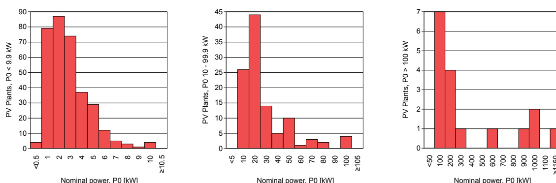
Figures 18, 19, 20, Distribution of the nominal power (P0) of the 461 grid-connected PV systems.
