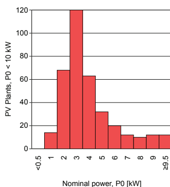
Figure 3, Datasets by nominal power, P0 < 10 kW.
