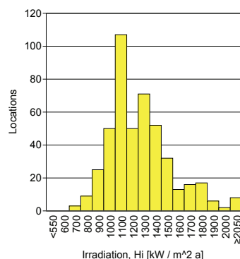
Figure 29, Distribution of in-plane irradiation.
