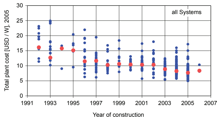
Figure 11, System cost in USD per watt over time.
