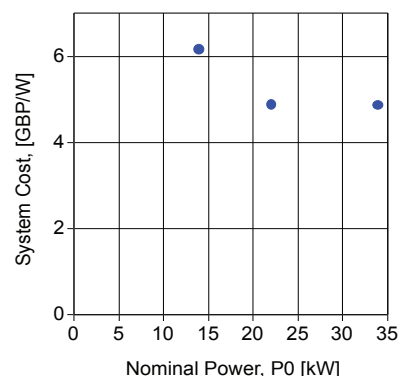
Figure 57, Overall specific cost data vs. nominal power.
