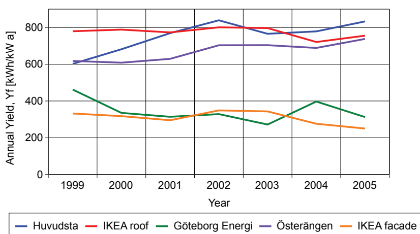
Figure 48, Annual yield of 5 Swedish systems all from 1999 to 2005. The values for Göteborg Energi and IKEA façade are considerably lower. Both these systems are façade installations using amorphous silicon. They were early experiments with this technology and the peak power is overestimated.
