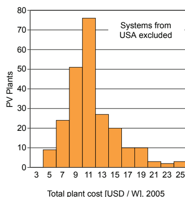
Figure 7, Plant cost, excluding USA.
