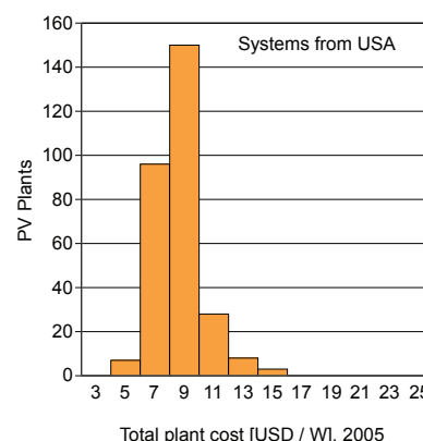
Figure 8, Plant cost, USA.
