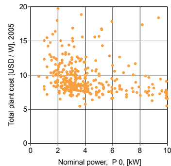
Figure 10, Plant cost to nominal power, P_0 < 10 kW.
