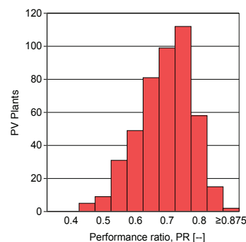
Figure 30, Distribution of the annual performance ratio.
