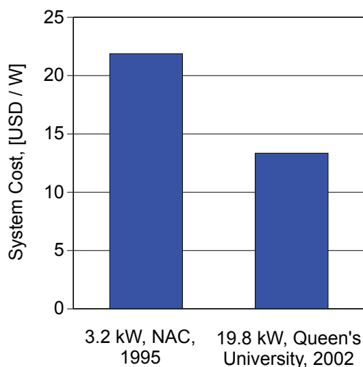
Figure 38, Comparison of the specific cost of the two Canadian PV systems.
