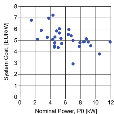
Figure 40, Specific plant cost as a function of installed power, German systems.
