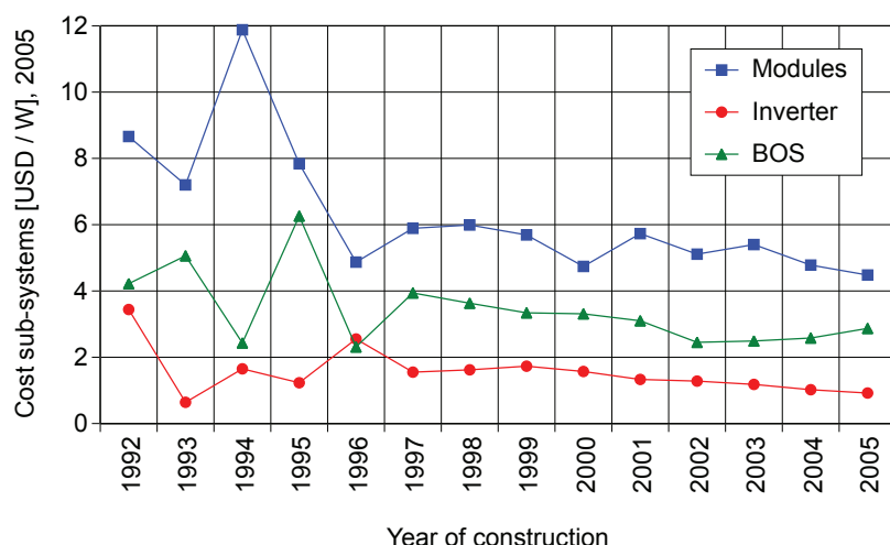
Figure 14, Cost sub-systems over time, 387 of 527 including 267 systems in the USA.
