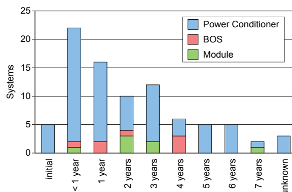
Figure III, Distribution of the operational year of first failure after installation from a survey of 725 small domestic PV systems in Japan.
