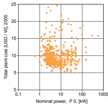
Figure 9, Plant cost to nominal power, logarithmic scale.
