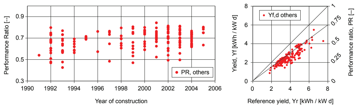
Figure 34, Performance ratio (PR) over time and final yield (Yf) vs. reference yield (Yr) all other countries.
