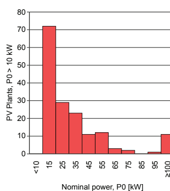
Figure 4, Datasets by nominal power, P0 > 10 kW.
