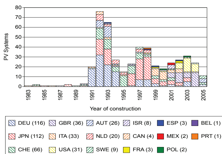
Figure 17, All 473 available grid-connected PV systems grouped by country and year of construction.
