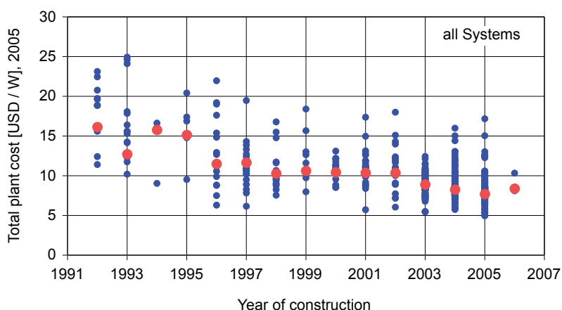
Figure 1, System cost in USD per watt over time, showing the values of each of the 527 grid-connected PV systems and the average value for each year from 1992 to 2006.
