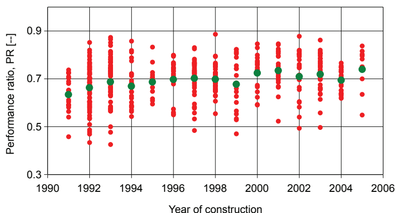
Figure II, Performance ratio over time of the 461 grid-connected PV systems built between 1991 and 2005. Showing the values for each system as well as the annual mean value.
