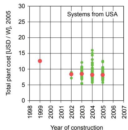
Figure 13, Cost over time, data from USA.
