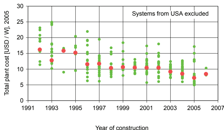
Figure 12, Cost over time, excluding data from USA.
