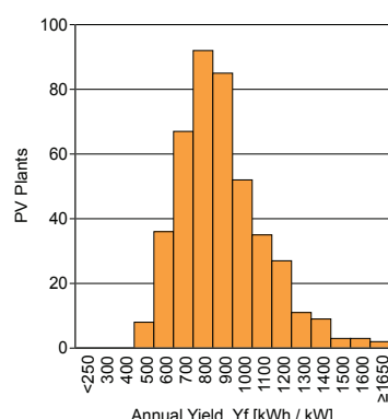
Figure 22, Annual yield (Yf), other systems.
