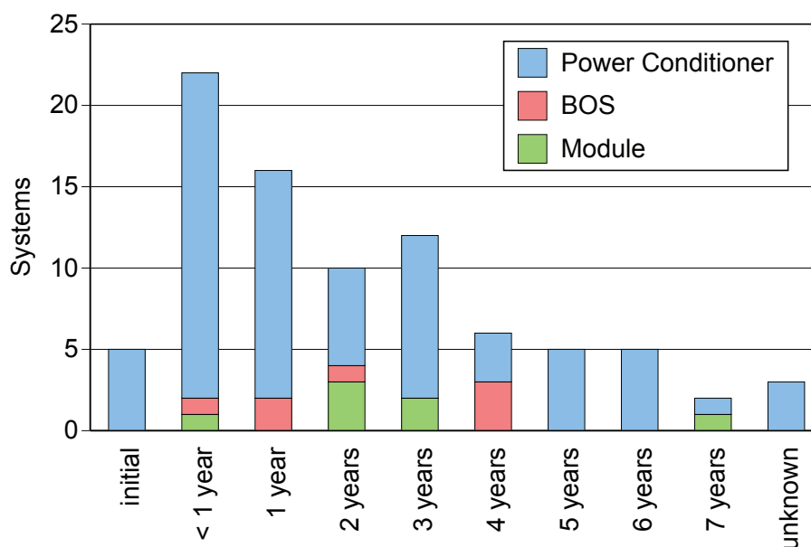
Figure 44, Distribution of operational year of the first failure after installation.
