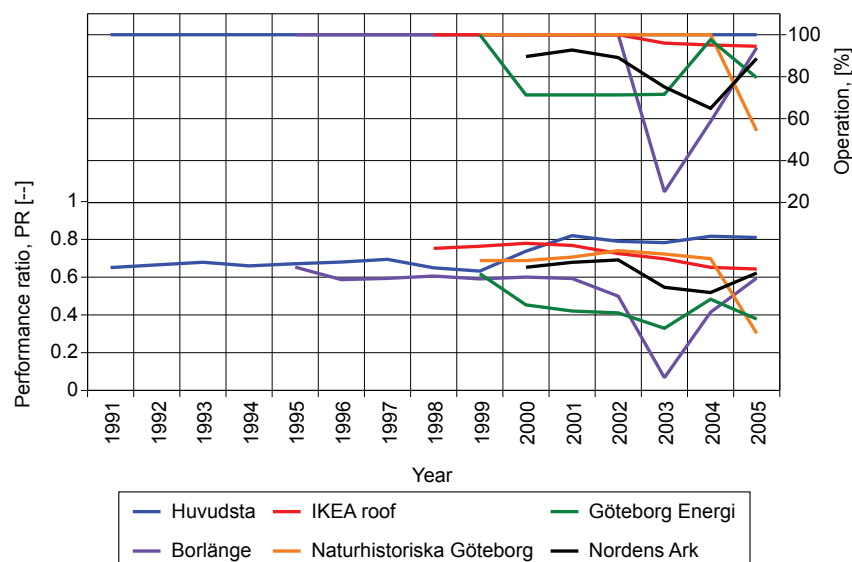
Figure 49, Performance over time for six Swedish grid-connected PV plants.
