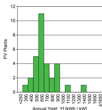
Figure 21, Annual yield, (Yf) façade systems.
