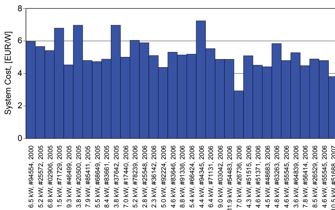
Figure 39, Specific plant cost of 33 grid-connected German residential PV systems, sorted by year of construction.
