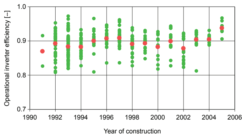
Figure 27, Annual operational inverter efficiency over time.
