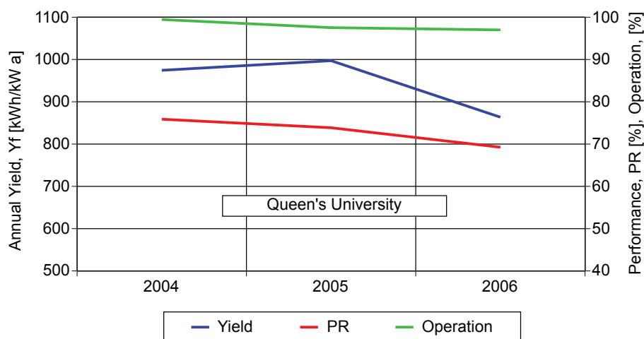
Figure 37, Annual yield, Performance and Operation of the Queen's University PV system from 2004 to 2006.
