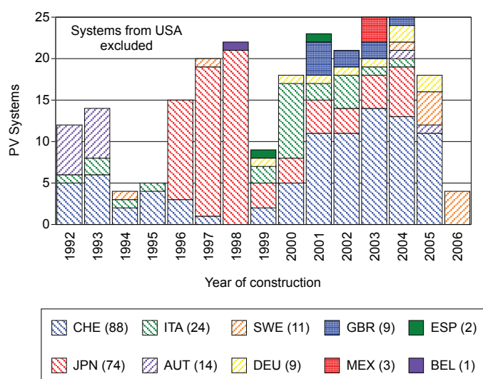
Figure 5, PV systems by country and year of construction.
