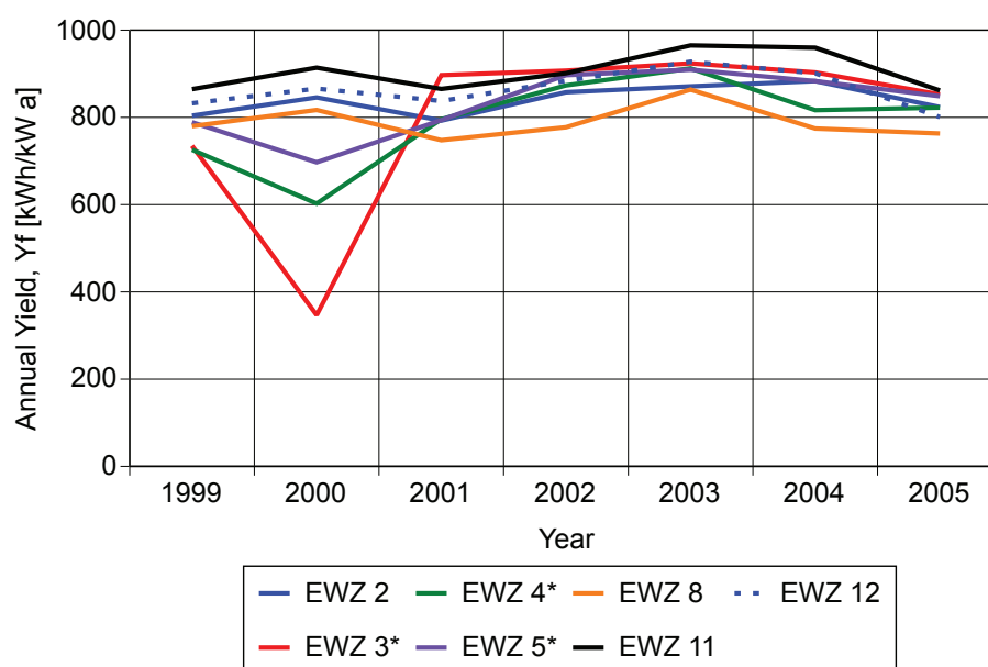
Figure 53, Annual yield ( Y_f ) of 7 PV systems in the Utility of Zürich, ewz PV programme.
