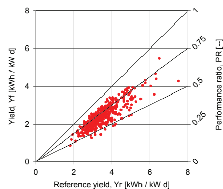
Figure 31, Final yield ( Y_f ) vs. reference yield ( Y_r ), all data.
